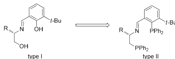
Scheme 1. O,N,O -Ligand (type I) and P,N,P -ligand (type II).
