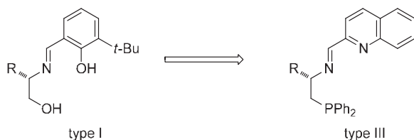
Scheme 4. O,N,O -Ligand (type I) to N,N,P -ligand (type III).
