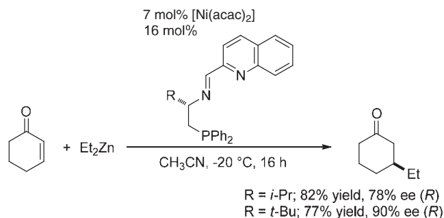
Scheme 10. Ni-Catalyzed asymmetric 1,4-addition.
