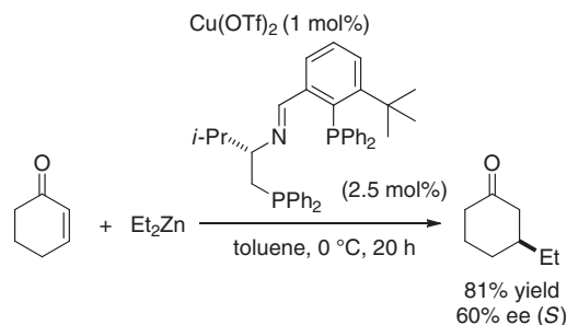
Scheme 3. Enantioselective 1,4-addition of diethylzinc to 2-cyclohexen-1-one.
