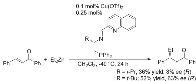
Scheme 11. Cu-Catalyzed asymmetric 1,4-addition of chalcone.
