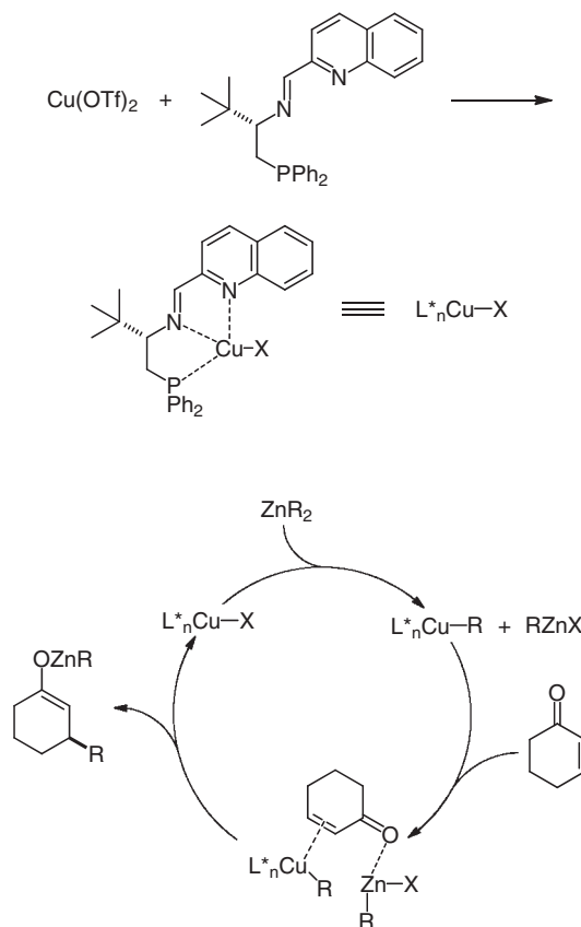
Scheme 6. Proposed catalytic cycle.
