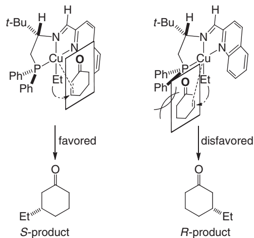
Scheme 7. Enantioselectivity of 1,4-addition.
