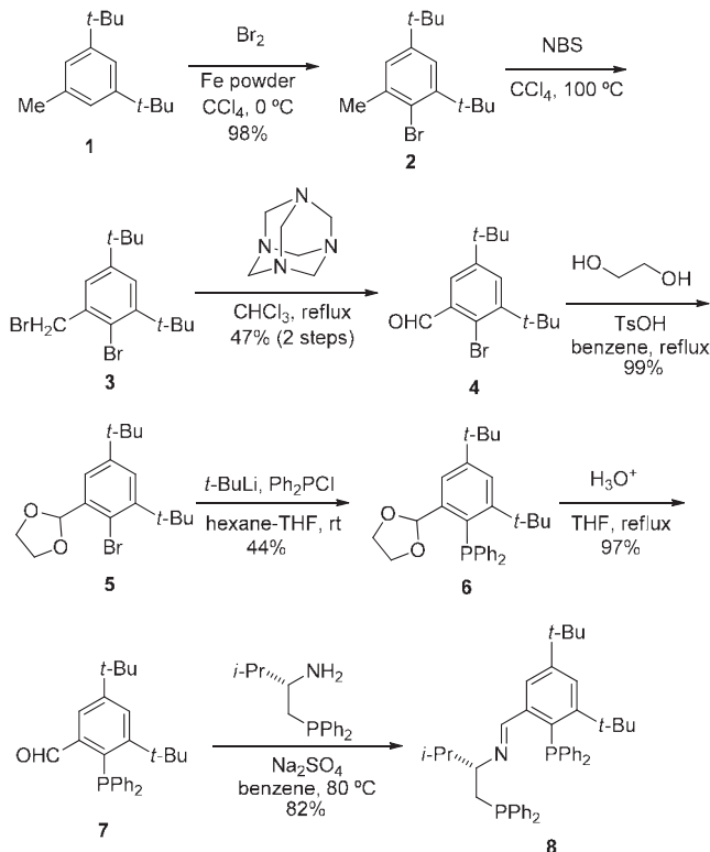
Scheme 2. Preparation of type II ligand.
