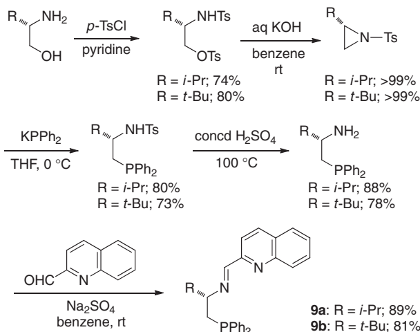
Scheme 5. Preparation of type III ligand.
