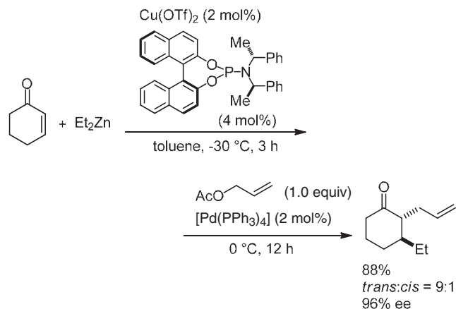
Scheme 8. Asymmetric conjugate addition (Feringa).
