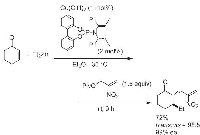
Scheme 9. Asymmetric conjugate addition (Alexakis).
